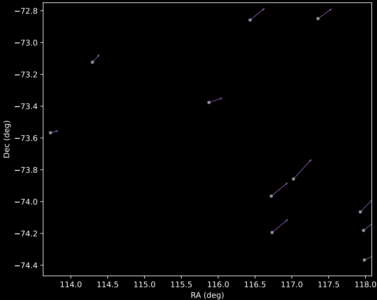
GALAH DR4 Cluster 8 Proper Motion Vectors (n=11)
