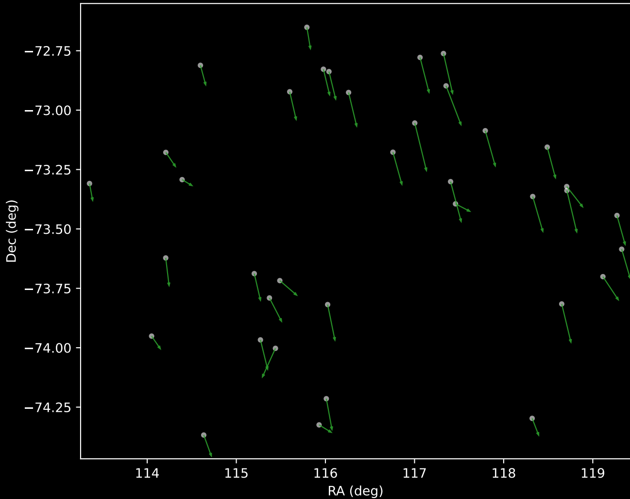
GALAH DR4 Cluster 4 Proper Motion Vectors (n=37)
