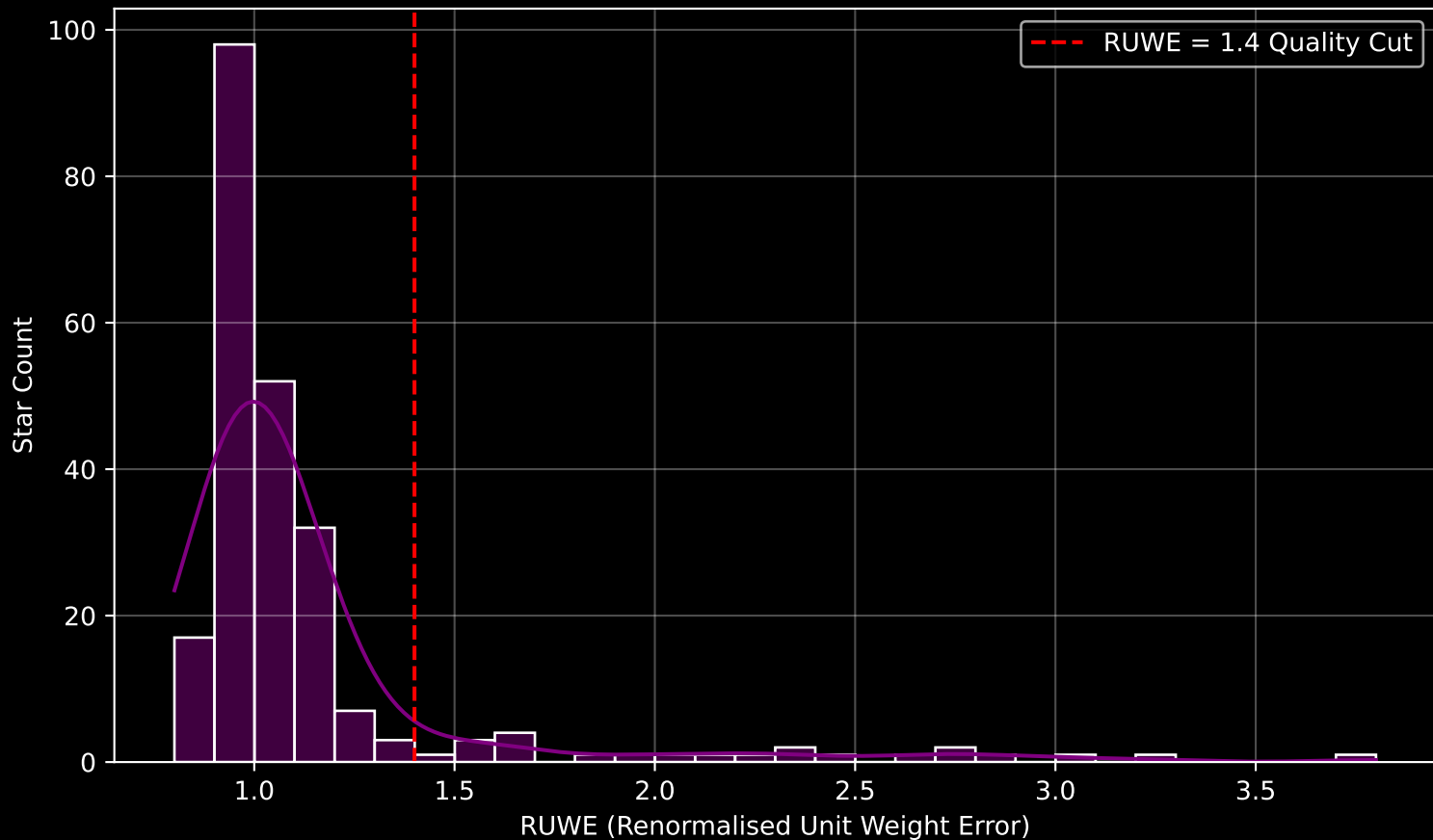
GALAH DR4 Field [92] RUWE Distribution (n= 232)
