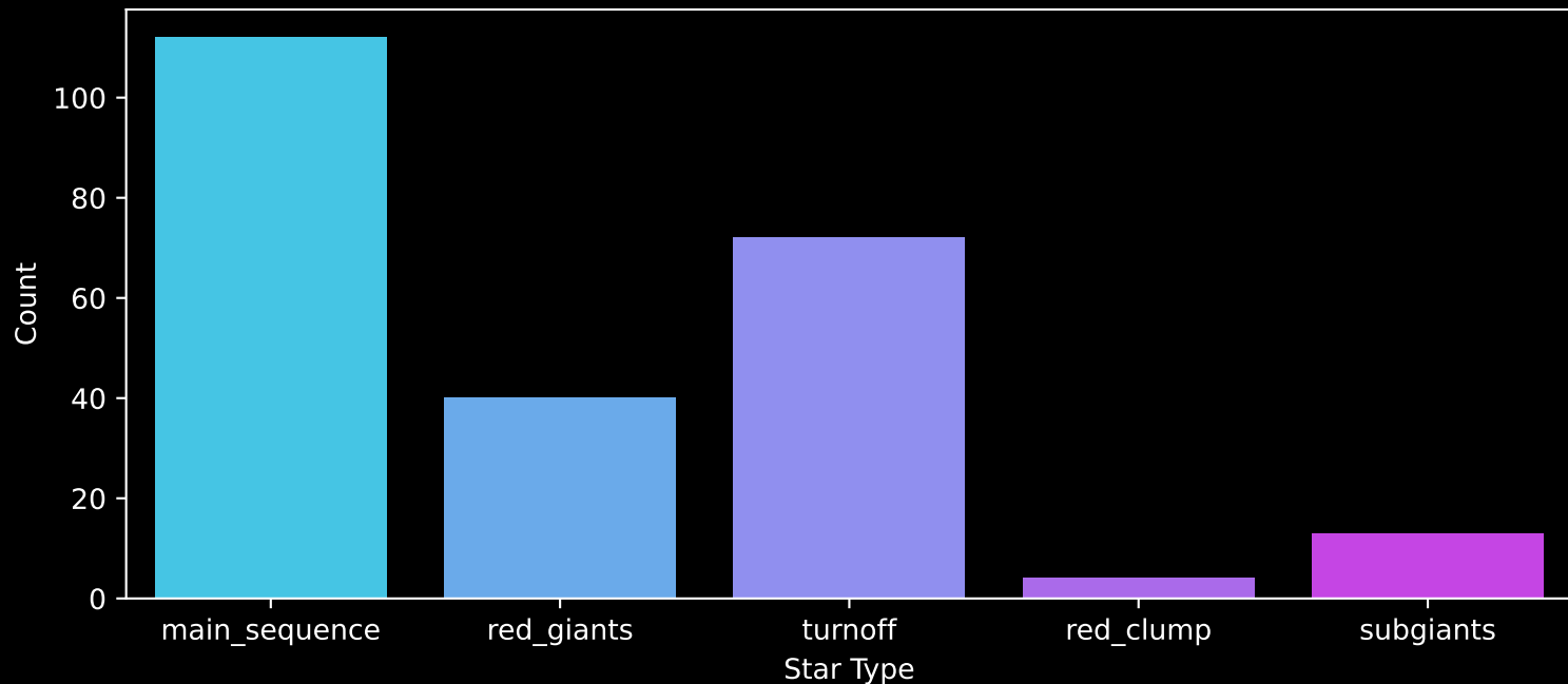
GALAH DR4 Field: [92] Count plot of Star Type
